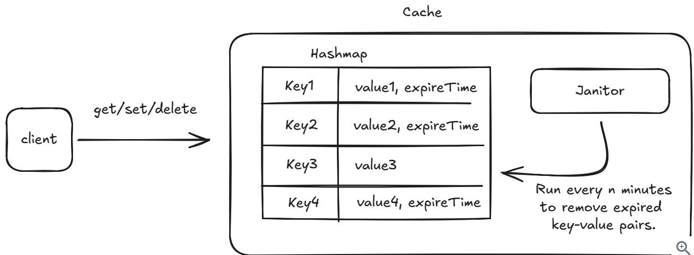
Simple Cache with TTLs
